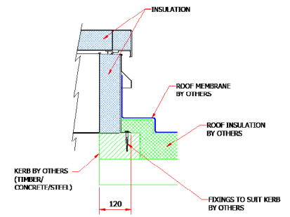
Typical Install
