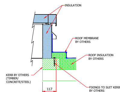
Typical Install
