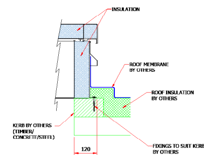
Typical Install
