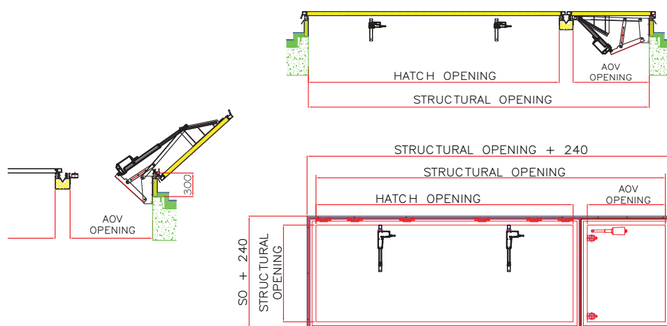
Typical Install
